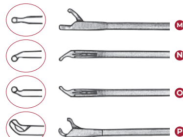
Round Cup Forceps extra delicate cup ø 1mm with cylindrical shaft
