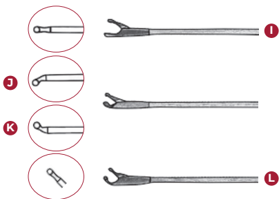
Miniature Round Cup Forceps Ø 1mm cup
