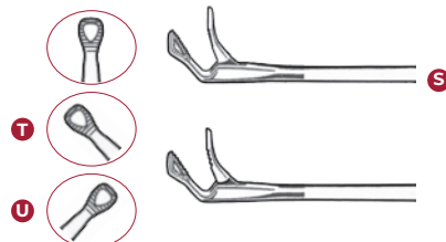
Triangular Grasping Forceps (heart shaped) fenestrated
