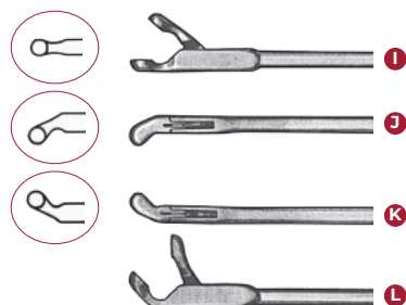
Round Cup Forceps ø 2.5mm with cylindrical shaft
