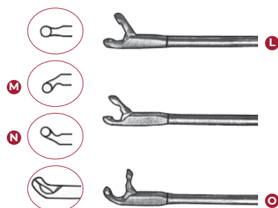
Round Cup Forceps ø 2.5mm cup
